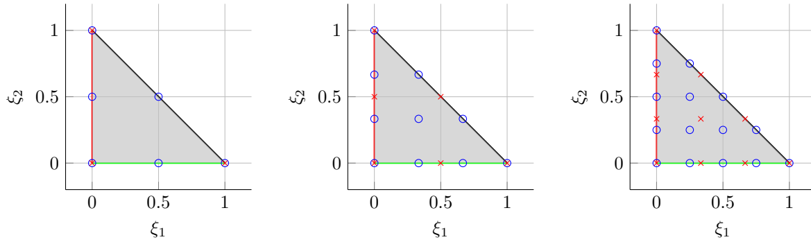
Figure 11: Mixed (velocity-pressure) triangular finite element in reference domain ( \xi_1 - \xi_2 space): \mathcal{P}^2 - \mathcal{P}^1 (quadratic approximation of velocity, linear approximation of pressure) ( left ), \mathcal{P}^3 - \mathcal{P}^2 (cubic approximation of velocity, quadratic approximation of pressure) ( center ), \mathcal{P}^4 - \mathcal{P}^3 (quartic approximation of velocity, cubic approximation of pressure) ( right ). The faces are numbered as: face 1 (—), face 2 (—), and face 3 (—). There is a velocity degree of freedom \mathbf{v}_i^e ( i = 1, \dots, N_{\text{nd}}^{\text{el}} ) at each ( \circ ) and a pressure degree of freedom P_i^e ( i = 1, \dots, \tilde{N}_{\text{nd}}^{\text{el}} ) at each ( \times ). For both sets of nodes, the numbering is inherited from the standard numbering in Figure 1.
