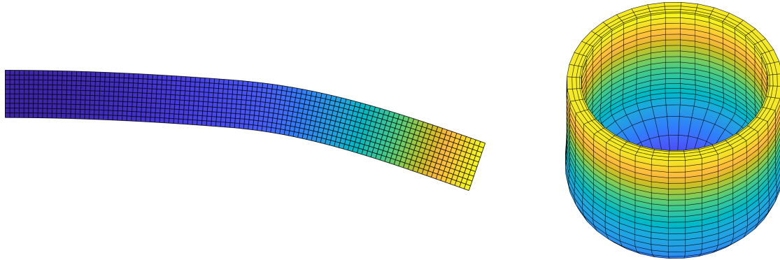
Figure 10: Solution of linear elasticity equations of multimaterial beam and hollow cylinder.
