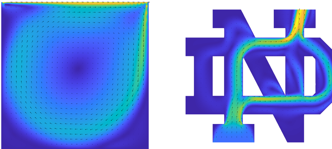
Figure 13: Solution of the incompressible Navier-Stokes equations: lid-driven cavity flow ( Re = 2000 ) and flow through ND logo ( Re = 1300 ).
