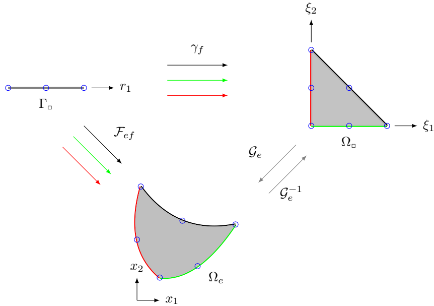
Figure 2: Mapping from (d-1) -dimensional reference simplex element ( \Gamma_\square ) to each face of the reference element ( \partial\Omega_{\square,f} ) ( \boldsymbol{\xi} = \gamma_f(\boldsymbol{r}) ), the mapping from the d -dimensional reference simplex element ( \Omega_\square ) to the physical element ( \Omega_e ) ( \boldsymbol{x} = \mathcal{G}_e(\boldsymbol{\xi}) ), and the composition mapping from the (d-1) -dimensional reference simplex element ( \Gamma_\square ) to each face of the physical element ( \partial\Omega_{ef} ) ( \boldsymbol{x} = \mathcal{F}_{ef}(\boldsymbol{r}) = \mathcal{G}_e(\gamma_f(\boldsymbol{r})) ).
