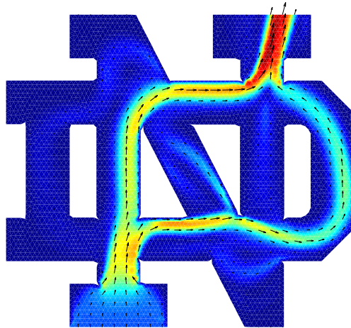
Figure 2.7: Solution of incompressible Navier-Stokes equation over the ND domain.
