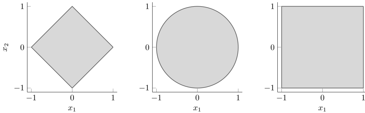
Figure 2.2: The gray region alone (without boundary (—)) defines the open unit ball B(0,1) , the union of the gray region and boundary (—) defines the closed unit ball \bar{B}(0,1) , and the boundary (—) alone defines the unit sphere S(0,1) corresponding to the one-norm \|\cdot\|_1 (left), two-norm \|\cdot\|_2 (center), and infinity-norm \|\cdot\|_\infty (right).
