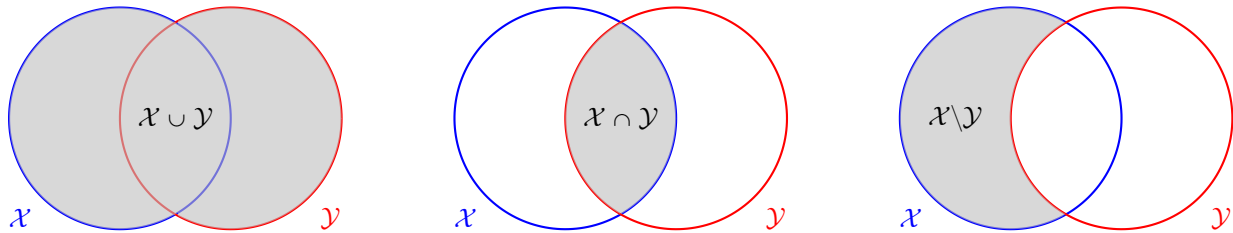
Figure 2.1: Illustration of set operations: union ( left ), intersection ( center ), and set difference ( right ).
