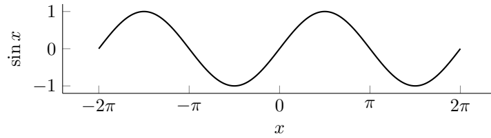
Figure 2.3: The sine function over the domain [-2\pi, 2\pi] .
