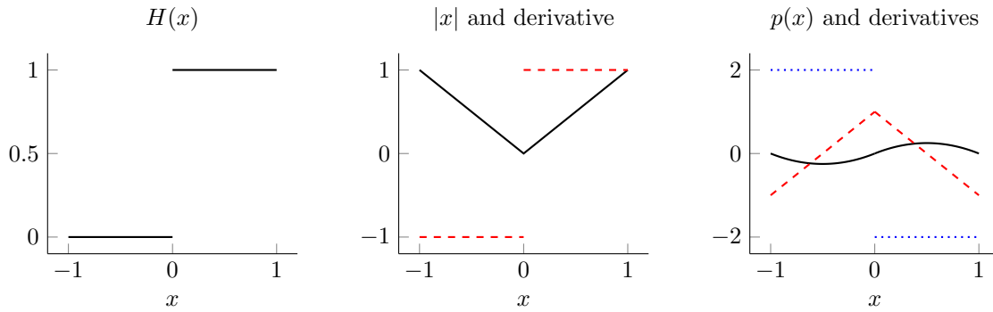
Figure 2.4: The value (—), first derivative (if exists) (---), and second derivative (if exists) (.....) of the Heaviside function (left), absolute value function (center), and piecewise polynomial function defined in (2.40) (right).
