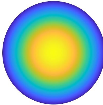
Figure 2.5: Solution of the Poisson equation over the disk.
